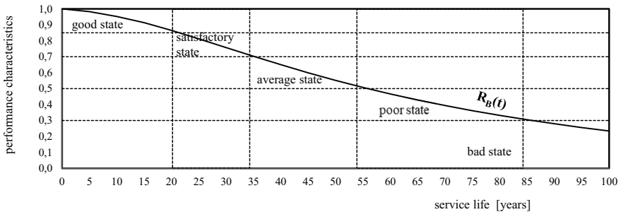
Fig. 1. Changes in performance characteristics of a building described by the PRRD model.
