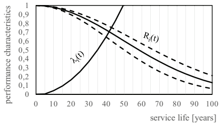
Fig. 3. Changes in the performance characteristics and damage intensity of wood ceilings
