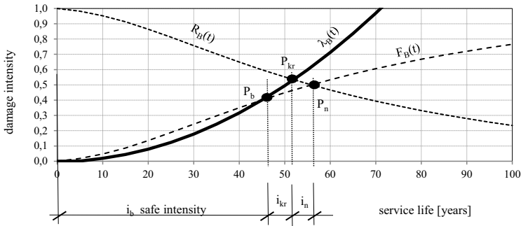
Fig. 6. Changes in the intensity of damage in an unrenovated building
