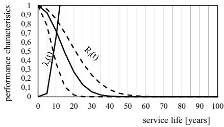
Fig. 5. Changes in the performance characteristics and damage intensity to gutters and downpipes
