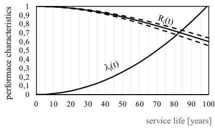
Fig. 2. Changes in the service properties and intensity of damage of masonry walls according to PRRD model.
