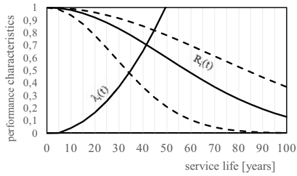
Fig. 4. Changes in the performance characteristics and damage intensity of plain roof tile
