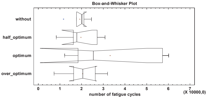
Fig. 10. Relations between number of fatigue cycles and amount of bitumen to glue the layers for specimens with glass geocomposite, T = 18° C
