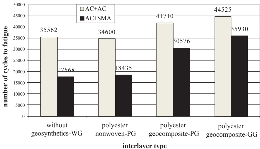
Fig. 6. Relation between number of fatigue cycles and type of interlayer, T = -2°C
