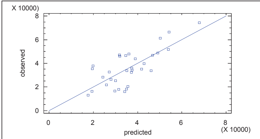
Fig. 15. Relations between observed and predicted number of fatigue cycles for specimens with geosynthetics
