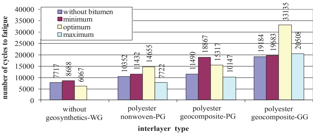
Fig. 5. Relation between fatigue life and type of interlayer for samples AC 12 with various amounts of bitumen spreading in interlayer, T = +18° C
