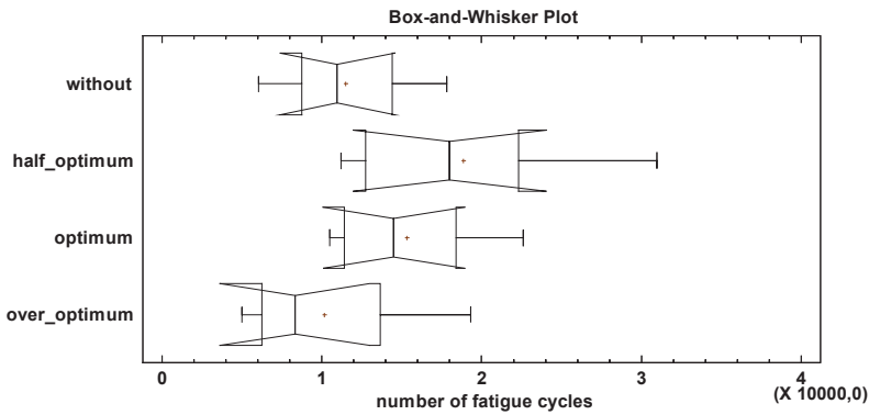
Fig. 9. Relations between number of fatigue cycles and amount of bitumen to glue the layers for specimens with polyester geocomposite, T = 18° C
