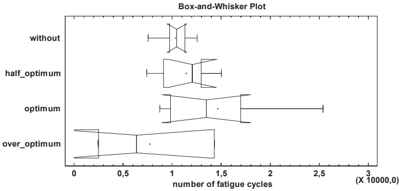
Fig. 8. Relations between number of fatigue cycles and amount of bitumen to glue the layers for specimens with polyester nonwoven, T = 18° C
