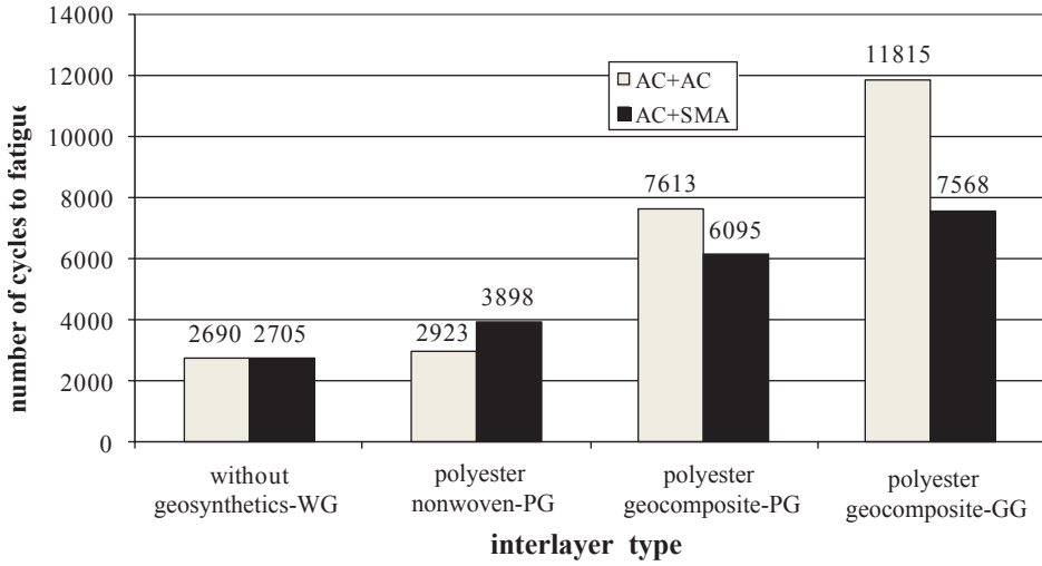
Fig. 4. Relation between type of interlayer and number of fatigue cycles, T = +18° C
