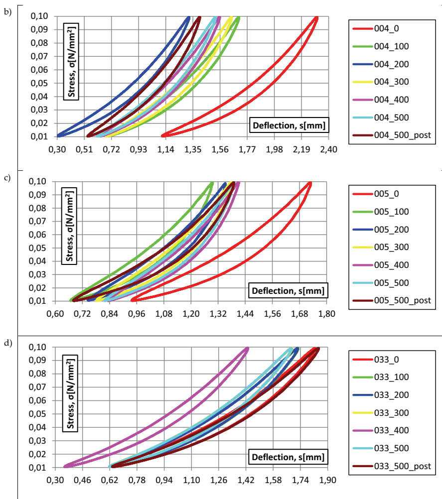
Fig. 5. Low frequency dynamic bedding modulus at 5 Hz for USP samples: a) 001; b) 004; c) 005; d) 033. The values and variations of the static bedding moduli (for two load ranges) and the low frequency dynamic bedding modulus at 5 Hz obtained in the fatigue tests for four analyzed USP samples are given in Table 1. It can be noticed that the biggest change of stiffness values for all four tested samples occurs after 100 thousand load cycles, afterwards the stiffness variations reach much smaller values.
