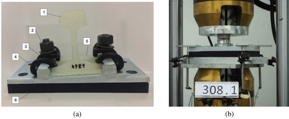
Fig. 24. Scheme of the discrete resilient rail fastening system for ballastless tracks: (a) View of the whole system; Symbols: 1 – Vignole rail with a 49E1 profile; 2 – alloy T-bolt and nut with washer; 3 – elastic rail clip/tension clamp type Skl 12; 4 – baseplate type Pm49; 5 – shaped rail pad type PAK; 6 – vibration isolation/baseplate pad (made of SBR granules – recycling material); (b) Test stand at the Faculty of Civil Engineering of the Warsaw University of Technology for determination of static and dynamic elastic characteristics of discrete elastic supports of the baseplate/rail: SBR-based specimen, 30 mm thick [12]
