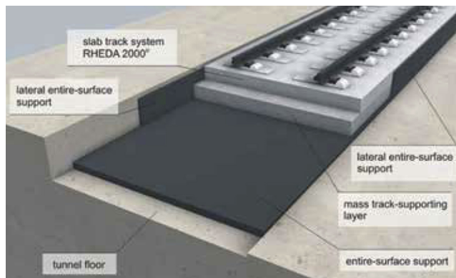
Fig. 10. System Rheda 2000 [3]
