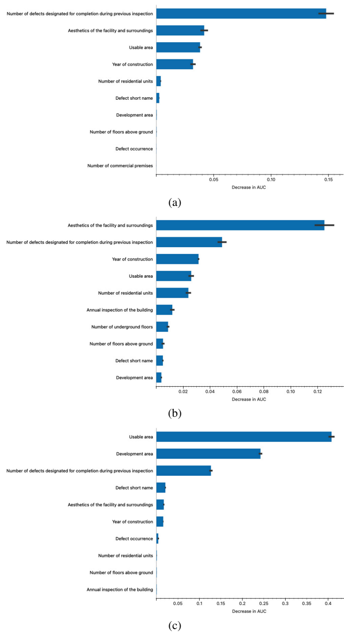
Fig. 2. The comparative feature importance analysis: (a) Gradient Boosting, (b) Random Forest, (c) k-NN
