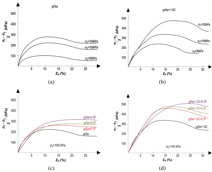
Fig. 5. Results of CD triaxial tests shown as half of the deviator stress- strain curves for: (a) gravelly sand at \sigma_{-3}' = 50\text{--}150 kPa, (b) gravelly sand with 1.5% of cement addition at \sigma_{-3}' = 50\text{--}150 kPa, (c) gravelly sand mix with fibres at 100 kPa, (d) gravelly sand/cement with 0.1, 0.2 and 0.3% of fibres at 100 kPa
