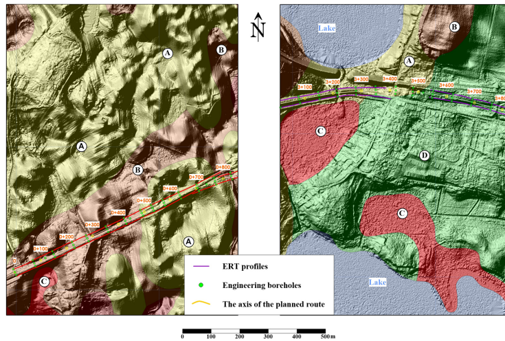
Fig. 5. Geological maps and ERT cross-sections. Legend for geological maps: A – sands and gravels, B – glacial tills, C – peats, D – clays, silts and lacustrine sands
