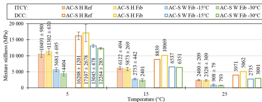
Fig. 4. The measured stiffness characteristics of the investigated high stiffness modulus asphalt concrete mixtures: IT-CY modulus (5, 15, 25^{\circ}\text{C} ), measured DCC complex modulus ( 5^{\circ}\text{C} ), DCC complex modulus from time-temperature shifted data (15, 25^{\circ}\text{C} )
