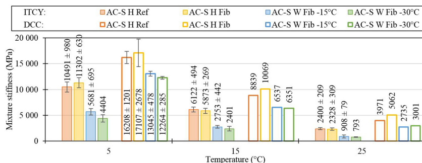
Fig. 3. The measured stiffness characteristics of the investigated surface course mixtures: IT-CY modulus (5, 15, 25^{\circ}\text{C} ), measured DCC complex modulus ( 5^{\circ}\text{C} ), DCC complex modulus from time-temperature shifted data (15, 25^{\circ}\text{C} )
