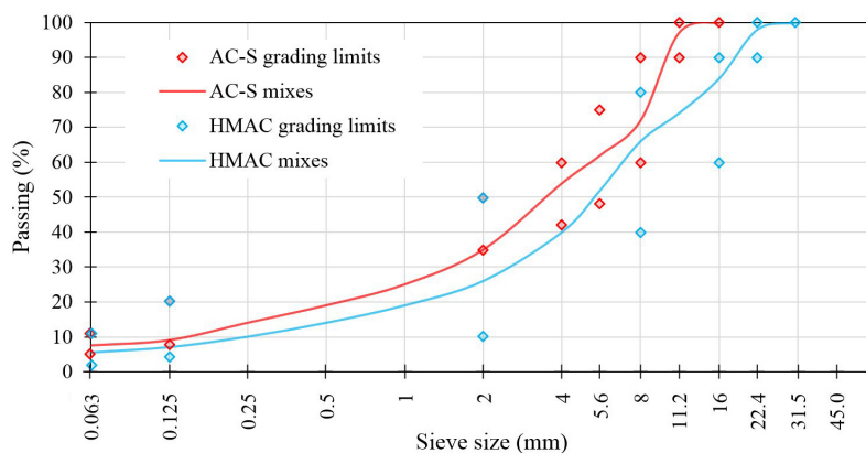
Fig. 1. Grading of the asphalt mixtures
