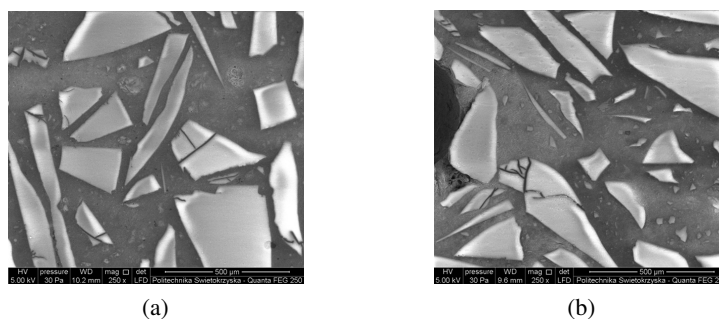
Fig. 6. Microstructure of mortars: (a) with the fly ash (V) and (b) with granulated blast furnace slag (S)
