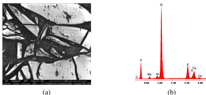
Fig. 5. Microstructure of mortars: (a) with CEM I cement (C2), (b) analysis of alkali-silica reaction products at point 1
