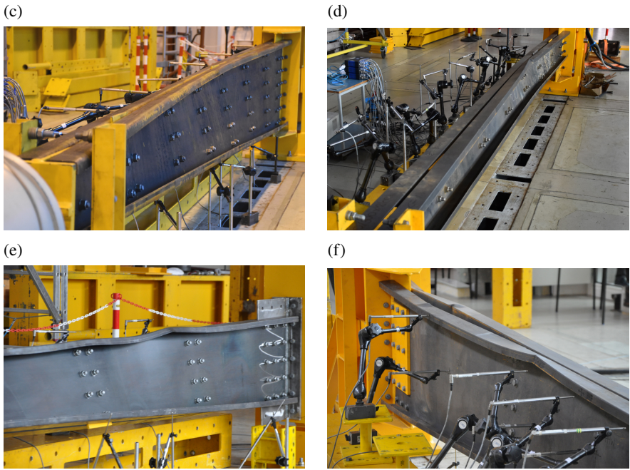
Fig. 6. Examples of failure modes of the tested specimens (description in the text)
