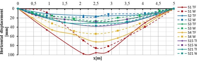
Fig. 7. Top flange (TF) and mid-height web (W) deformations in samples in compression at maximum load
