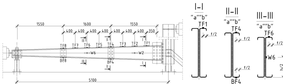
Fig. 4. Arrangement of foil strain gauges in sample S18
