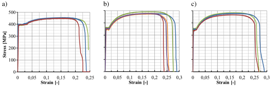
Fig. 5. Stress-strain curves from coupon tests for: (a) 2 mm, (b) 4 mm, and (c) 6 mm thickness group.
