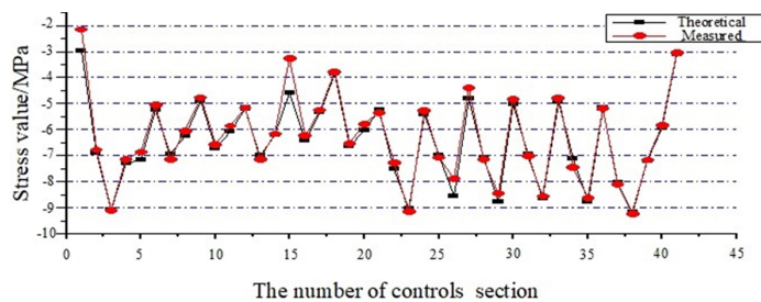
Fig. 17. Stress diagram of the upper edge of the control section during the bridge formation stage
