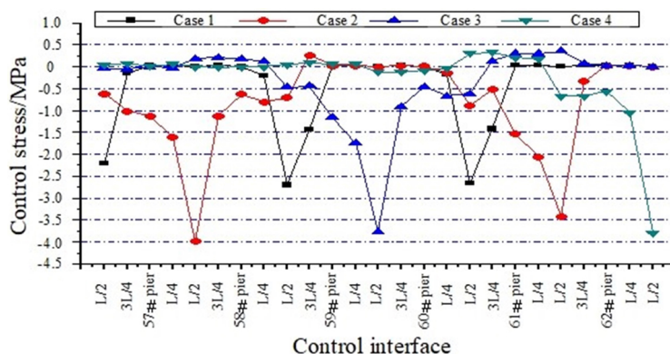
Fig. 7. Variation of stress at the upper edge of the control section under each working condition
