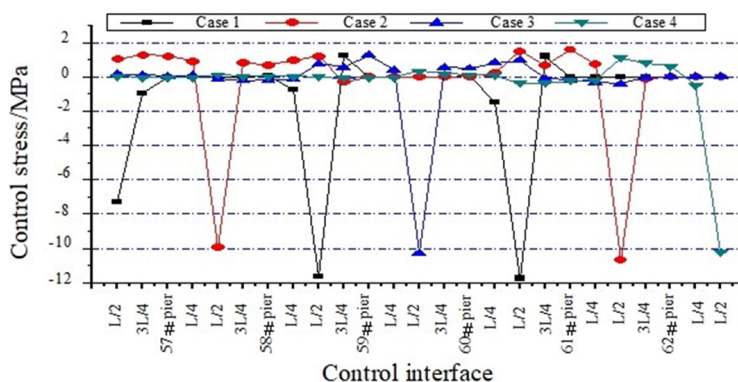
Fig. 8. Stress variation diagram of the lower edge of the control section under each working condition
