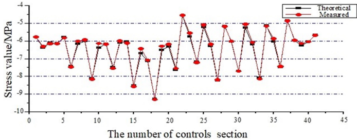
Fig. 18. Stress diagram of the lower edge of the control section during the bridge formation stage
