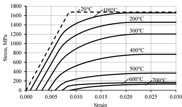
Fig. 5. Diagrams of the stress-strain relationship at high temperature suitable for estimating the total elongation of Y1860S7 tendons in members exposed to fire conditions
