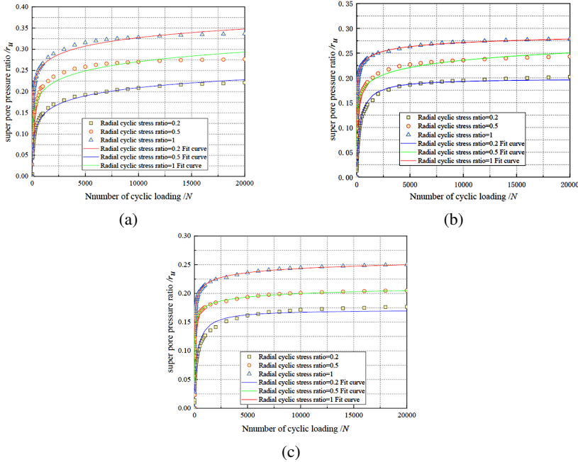
Fig. 8. Pore pressure fitting curves under different radial cyclic stress ratios; (a) Effective confining pressure = 150 kPa, (b) Effective confining pressure = 200 kPa, (c) Effective confining pressure = 250 kPa
