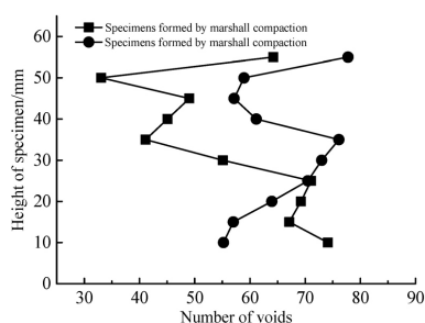
Fig. 18. Distribution of the number of voids along the height of specimen
