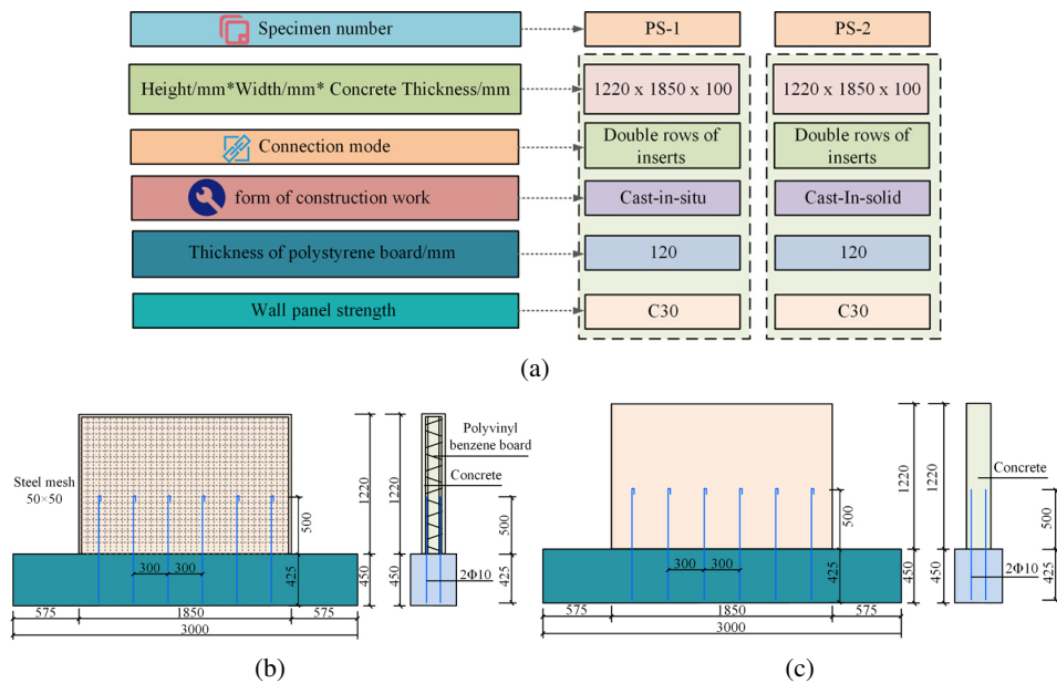
Fig. 1. Cast-in-situ shear wall specimen design parameters and detailed structure diagram; (a) Parameters of cast-in-place shear wall specimen, (b) Detailed construction diagram of PS-1, (c) Detailed construction diagram of PS-2
