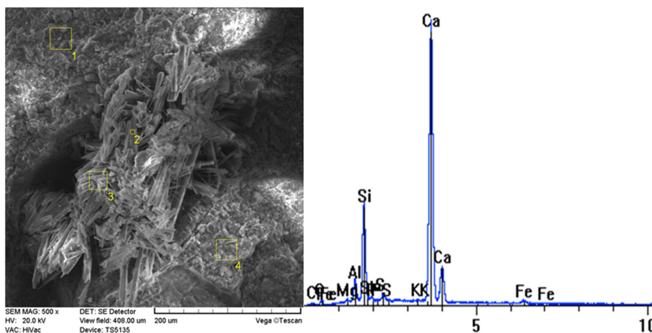
Fig. 14. Analysis of upper part of floor (sample B) riched in ettringite. X-ray photography, the analysis of elements occurrence
