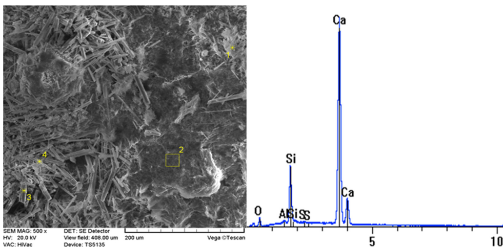
Fig. 15. Analysis of bottom part of floor (sample B) riched in ettringite. X-ray photography, the analysis of elements occurrence
