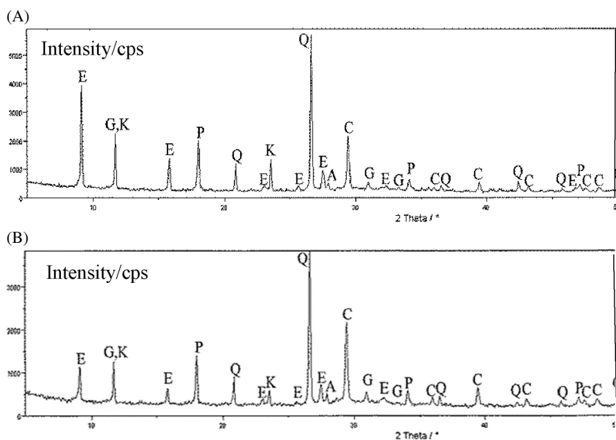
Fig. 11. Phases formations during long time hydration of portland cement concrete. Symbols of concrete phases: A – albite, Q – quarc, C- calcite, E – ettringite, G- gipsum, K – carboaluminate, P – portlandite
