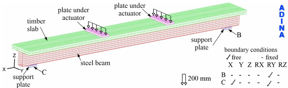
Fig. 7. The numerical model in ADINA
