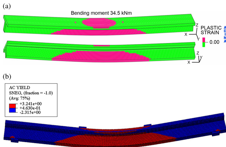
Fig. 11. The yield strength achieved in the omega girder and the resistance of the LVL achieved on the top and bottom edges of the slab: (a) in the ADINA program ( M = 34.5 \text{ kN} \cdot \text{m} ); (b) in the Abaqus program ( M = 36.0 \text{ kN} \cdot \text{m} )
