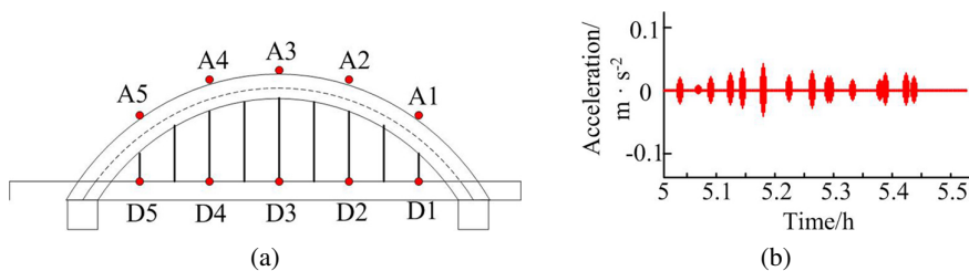
Fig. 4. Collection points and acceleration signal time history: (a) Layout diagram of acceleration sensors, (b) Time history of bridge measured acceleration signal
