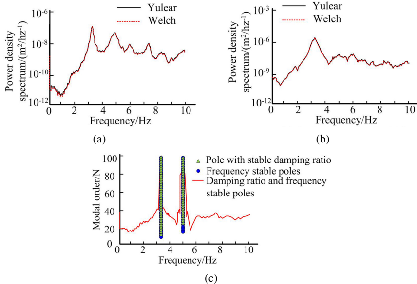
Fig. 5. Natural frequency identification of civil engineering bridge structures in two cases and stability map after SSI method processing: (a) Environmental spectrum analysis results, (b) Analysis results of vehicle load spectrum, (c) Stability map obtained by SSI
