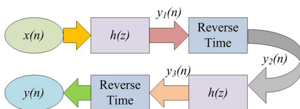
Fig. 3. FRR zero phase filtering process
