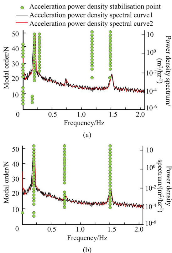
Fig. 7. PSD analysis results of acceleration data in various channels of high-rise buildings: (a) Stable graph obtained from unimproved SSI, (b) Stable graph obtained from improved SSI
