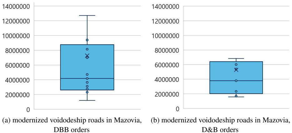
Fig. 6. Box-plots for the C4 comparison samples: (a) DBB orders, (b) D&B orders
