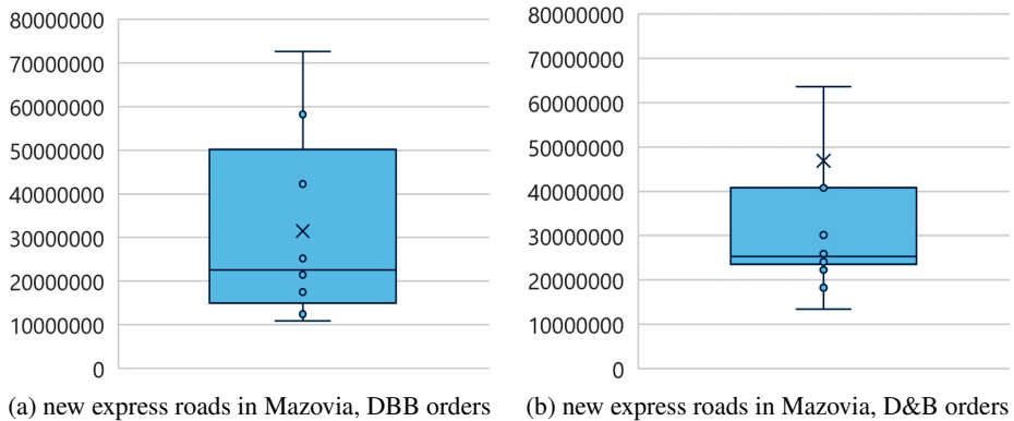
Fig. 5. Box-plots for the C1 comparison samples: (a) DBB orders, (b) D&B orders (outliers are excluded in b)
