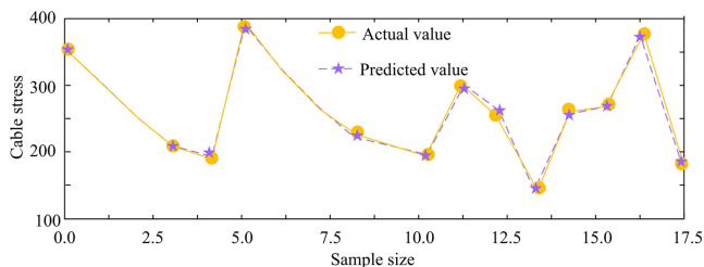
(b) Comparison of the predicted value and the actual value of the cable stress by intelligent algorithm
