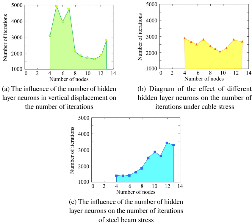
Fig. 5. Schematic diagram of the influence of different mechanical parameters and different number of hidden layer neurons on the number of iterations
