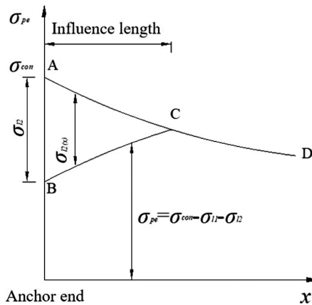
Fig. 1. Calculation diagram for stress loss considering reverse friction
