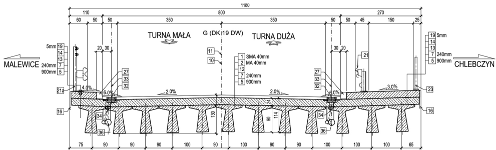
Fig. 3. Cross-section of the WD-8 viaduct
