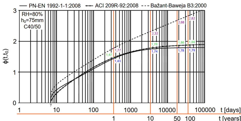
Fig. 2. Comparison of creep coefficients of concrete \phi(t, t_0) [27] according to PN-EN [10], ACI [24] and B3 [20] for concrete class C40/50, RH=80%
