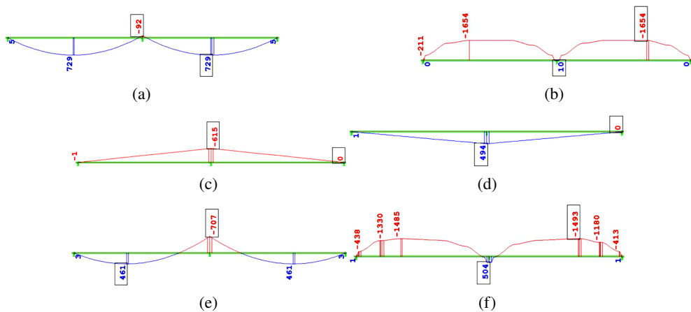
Fig. 4. Diagrams of the bending moment M_y [kN-m] caused by: (a) self-weight in the continuous system immediately after monolithization of the joints, (b) concrete creep from self-weight over 100 years of use, (c) self-weight after redistribution caused by concrete creep (d) prestressing of prefabricated elements in the continuous system immediately after monolithization of the joints, (e) concrete creep due to prestressing force over 100 years of use, (f) prestressing of prefabricated elements after redistribution caused by concrete creep
