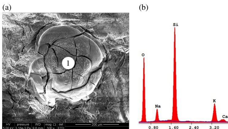
Fig. 7. (a) Sodium-potassium-calcium silicate gel in metahalloysite mortar, (b) gel composition – EDS analysis at point 1
