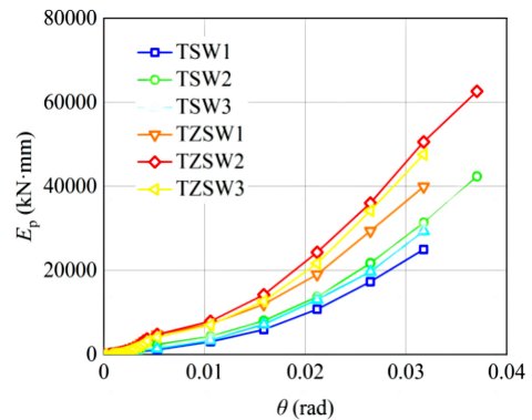
Fig. 9. Accumulated energy dissipation curves
