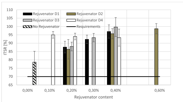
Fig. 8. Water sensitivity test result depending on rejuvenator type and content
