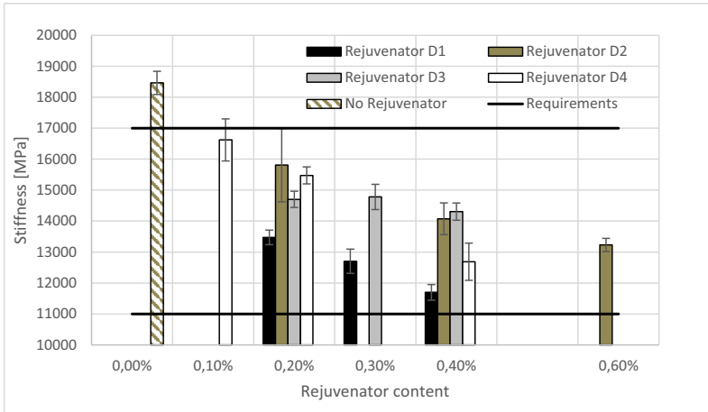
Fig. 6. Stiffness value depending on the rejuvenator type and content
