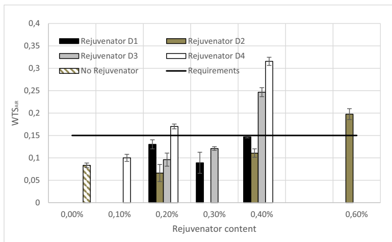
Fig. 5. WTS_{AIR} value depending on the rejuvenator type and content
