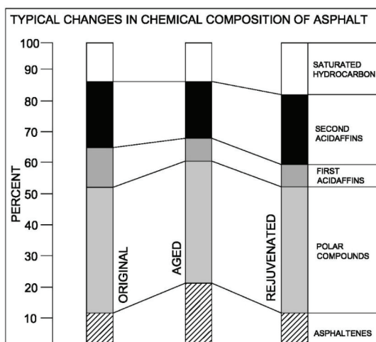
Fig. 1. Changes in the chemical composition of bitumen due to ageing and following rejuvenation [22]
