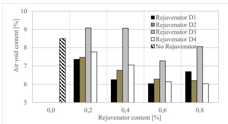
Fig. 3. Air voids content determined on Marshall specimens
