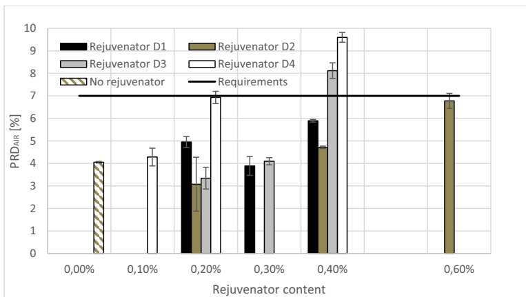
Fig. 4. PRD_{AIR} value depending on the rejuvenator type and content
