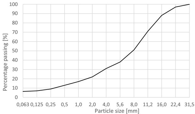
Fig. 2. Particle size distribution of the HMA mixture sampled from base course layer as RAP material for the main tests as per EN 12697-2
