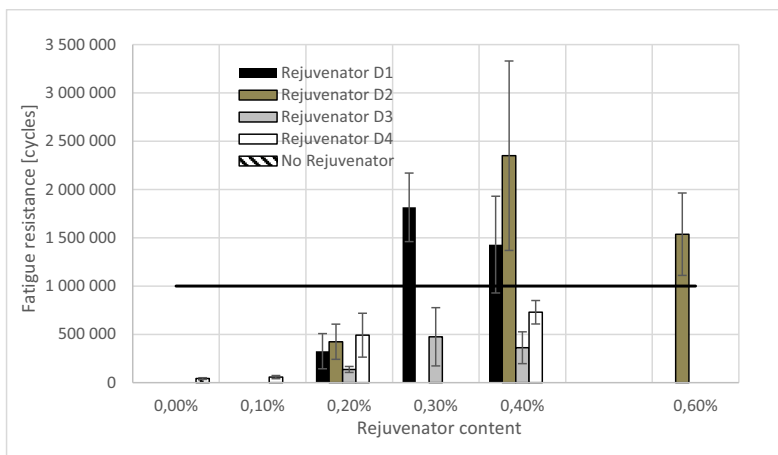
Fig. 7. The fatigue resistance level depending on rejuvenator type and content
