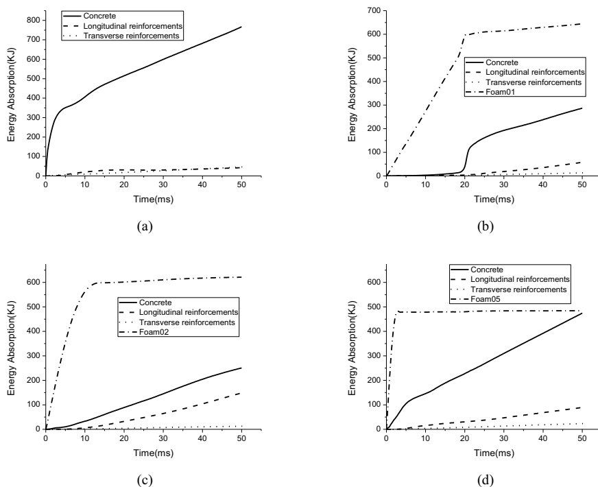
Fig. 8. The energy absorption history of RC columns components: (a) The naked column without safeguard; (b) The safeguarded column by the foam01 with relatively density 0.1; (c) The safeguarded column by the foam02; (d) The safeguarded column by the foam05.
