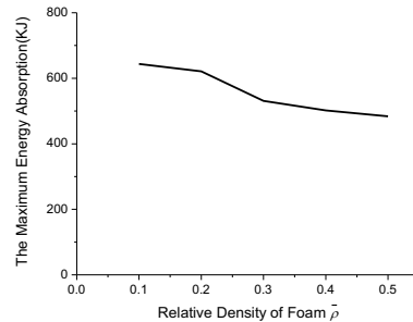
Fig. 10. The variation of the maximum energy absorption of the foams with relative density
