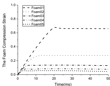
Fig. 5. The nominal compression strain of foams-time history
