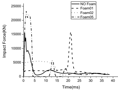
Fig. 6. The resultant impact force-time history
