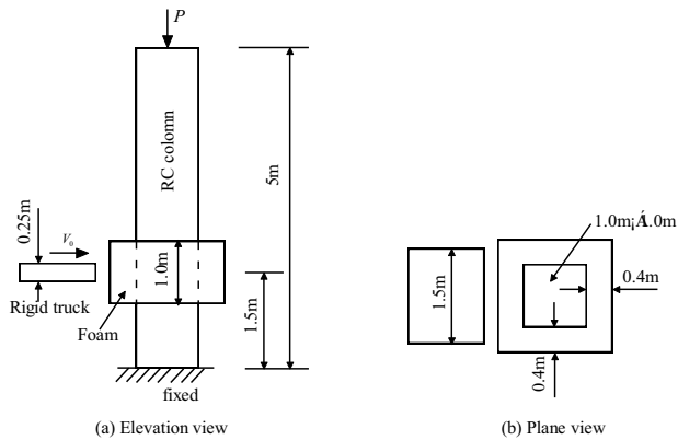
Fig. 1. The geometric configurations of rigid truck impact with foam safeguarded RC column
