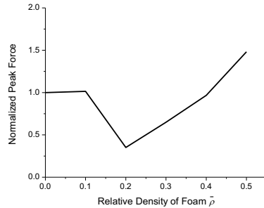
Fig. 7. The variation of the normalized peak forces with relative density of the foams
