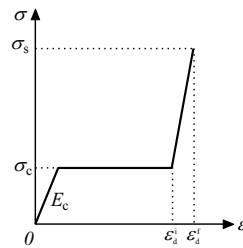
Fig. 2. Simplified uniaxial compression curve of foam materials
