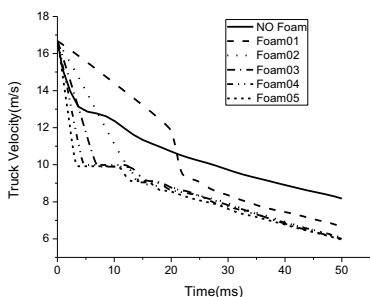
Fig. 3. The truck velocity-time history
