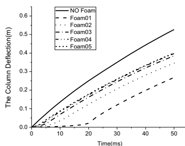
Fig. 4. The column deflection-time history along the impact direction
