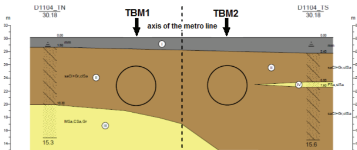
Fig. 6. Geological scheme of the section no. 1104
